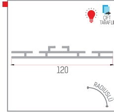
120 mm (1,328 kg/m)
