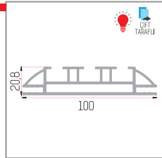
100 mm (1,317 kg/m)
