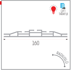
160 mm (1,854 kg/m)
