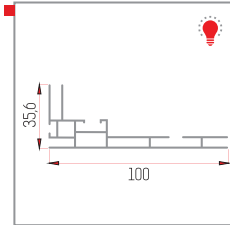
100 mm (1,144 kg/m)
